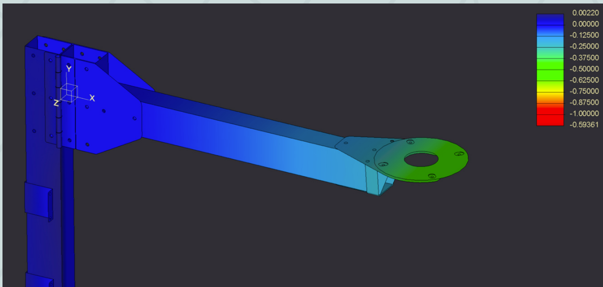
Visualisation of stress test under maximum load
